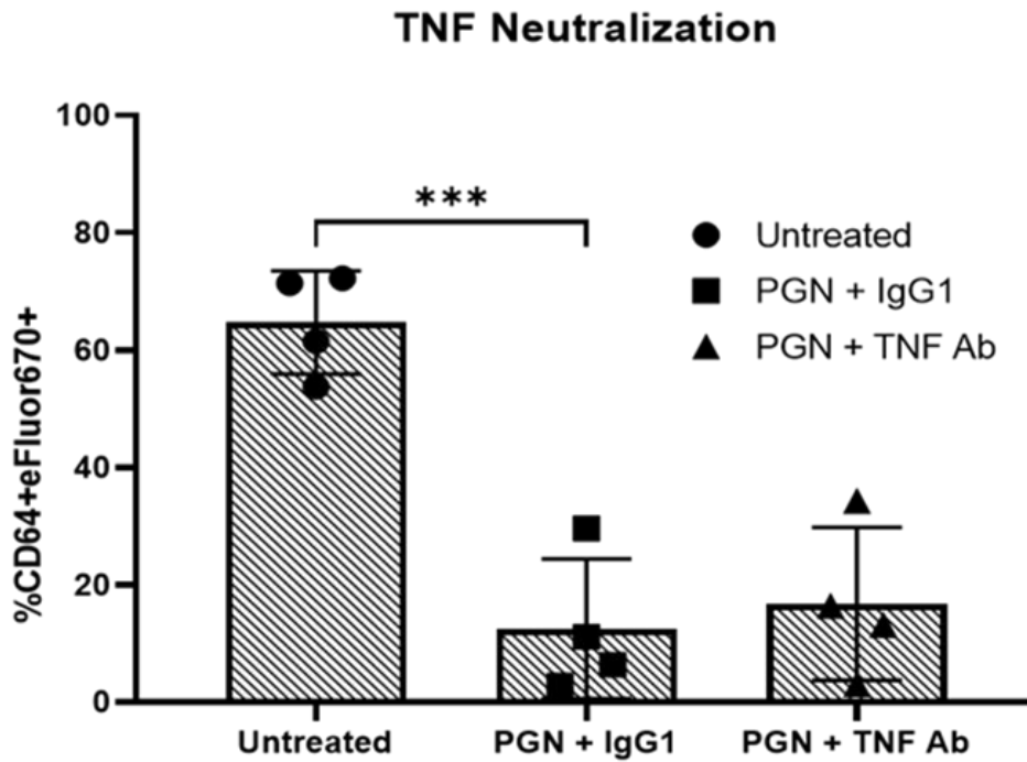
Supplemental Figure 4: TNF neutralization does not rescue PGN-induced defects in efferocytosis. Percentage of CD64+ M \Phi containing apoptotic eFluor670-labeled PMN treated with 6 \mu g/mL of either an IgG isotype control ( \beta -Galactosidase, InvivoGen Cat#: bgal-mab1) or human anti-TNF (IgG1, InvivoGen, Cat#: htnf-mab1) antibody in the presence of 10ug/mL PGN for 24 hrs. 4 independent donors analyzed by one-way ANOVA with Dunnet's multiple comparison.
