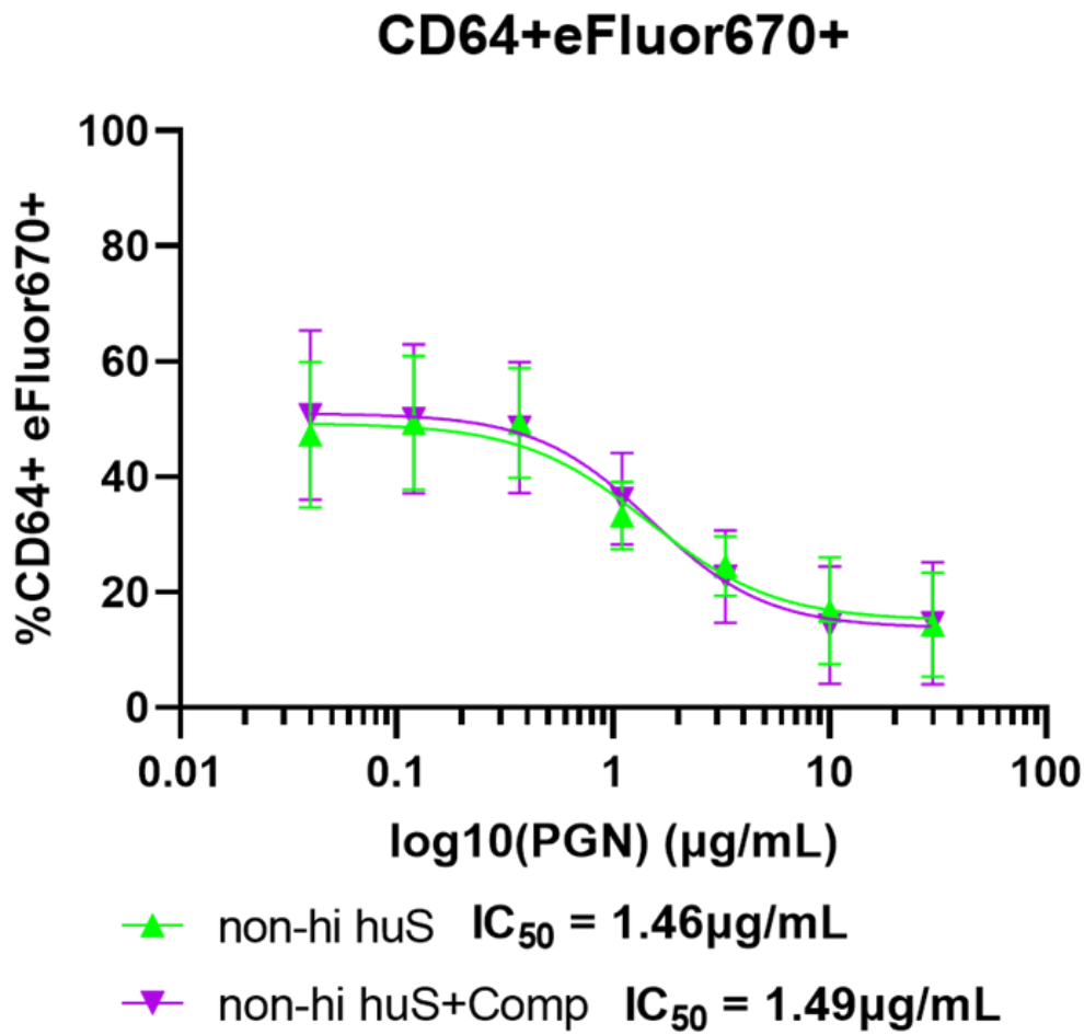
Supplemental Figure 2: Dose response of PGN on MΦ efferocytosis from non-hi huS or non-hi huS+ Compstatin conditions from 3 independent donors (30µg/mL-0.04µg/mL). Data was log(10)-transformed and graphed using a non-linear fit model in Prism. Dose-response curve was used to calculate IC_{50} .
